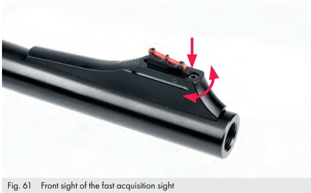
Fig. 61 Front sight of the fast acquisition sight
