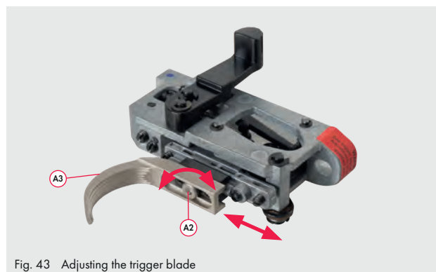
Fig. 43 Adjusting the trigger blade
