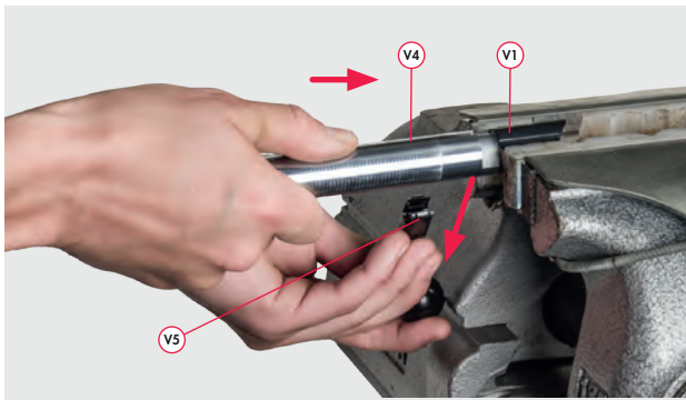
Fig. 23 Pulling out the bolt handle
