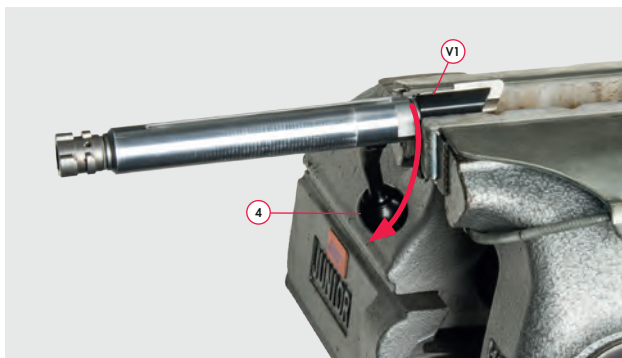
Fig. 13 Alternatively, the bolt can be clamped for these steps
