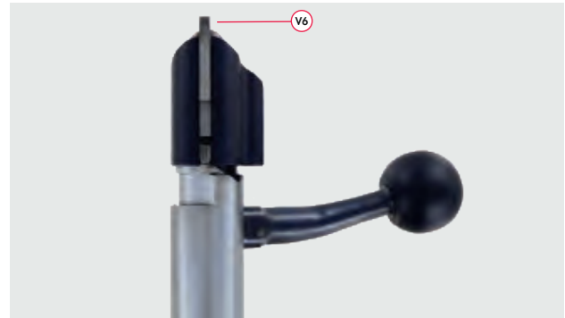
Fig. 19 Bolt in cocked position after removal, Plunger lug [V6] visible
