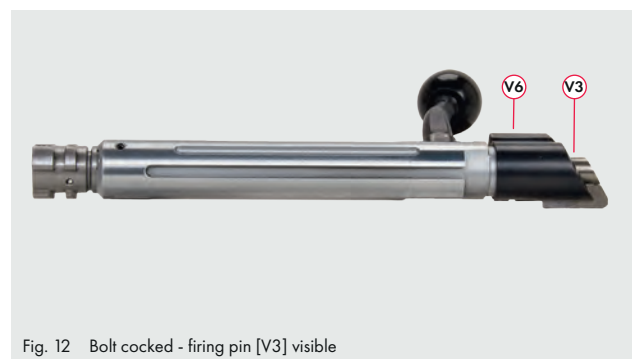
Fig. 12 Bolt cocked - firing pin [V3] visible
