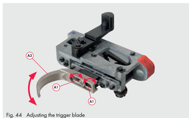
Fig. 44 Adjusting the trigger blade
