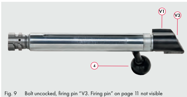
Fig. 9 Bolt uncocked, firing pin "V3". Firing pin "V3" on page 11 not visible
