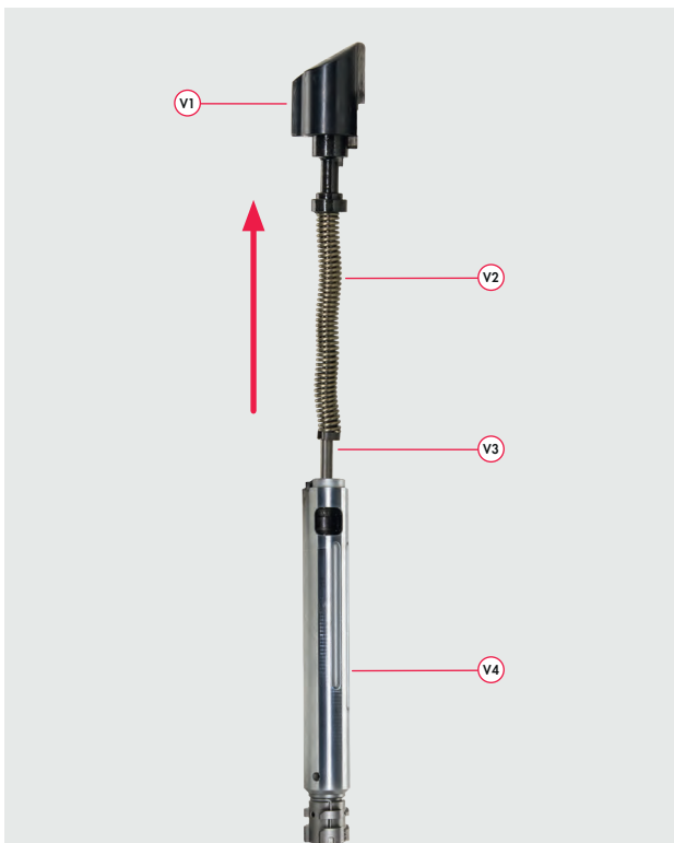
Fig. 24 Pulling out firing pin with spring
