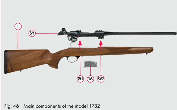
Fig. 46 Main components of the model 1782
