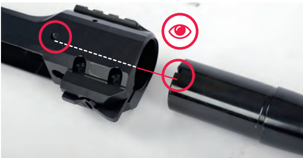
Fig. 58 During assembly, the groove and guide pin must be flush
