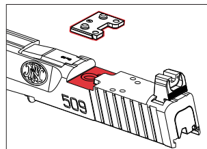
FN optics mounting system.
