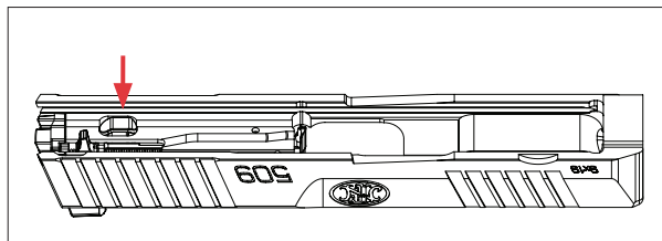
Striker block.
