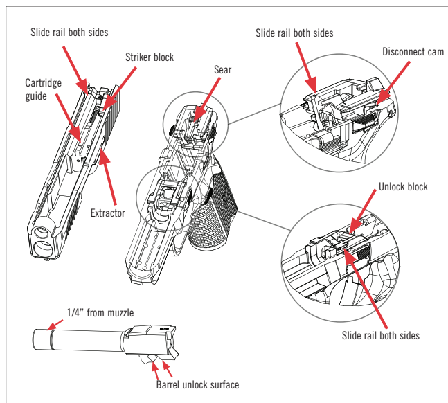
Lubrication Points.
