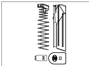
Magazine components.
