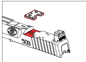
FN's patented Low Profile Optics Mounting System, U.S. Patent No. 10,352,654
