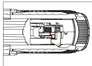
Trigger disconnect.
