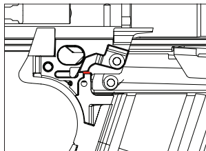
Drop safety.
