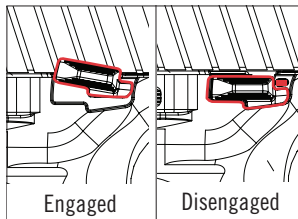
Manual safety.
