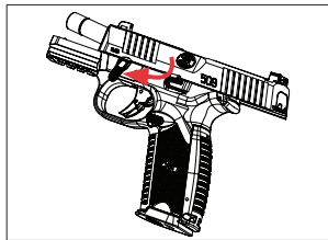
Takedown lever rotated.
