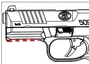
Accessory rail.
