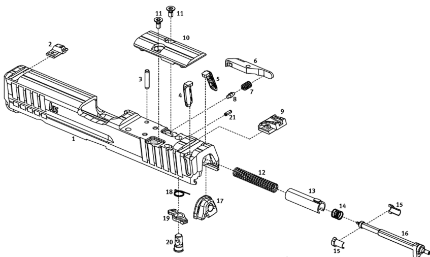
Figure 68 VP Optic Ready Slide Exploded Diagram
